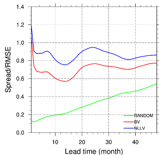
Fig. 14 Ratio of the ensemble member spread (represented by the averaged standard deviations of the model ensembles) and the RMSE of the ensemble mean shown as functions of lead time for different ensemble schemes: random perturbation method (green line), BV method (red line), and NLLV method (blue line). Values close to 1 represent good results
