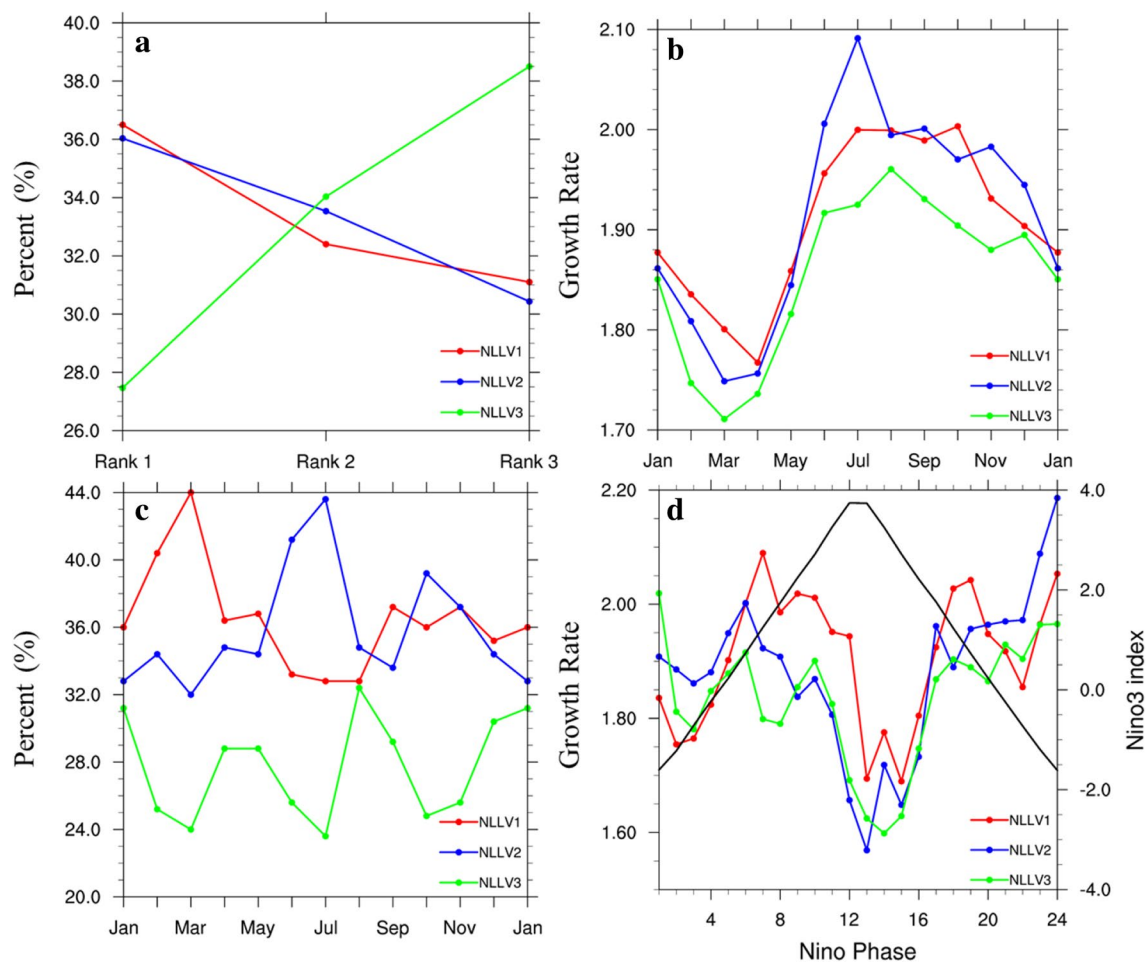
Fig. 6 Percentage of the first three NLLVs in the position of the corresponding rank (a), the growth rates of the first three NLLVs for different seasons (b), the percentage of the first three NLLVs as the fastest growth direction for different seasons (c) and the average growth rate of the first three NLLVs as a function of the ENSO
