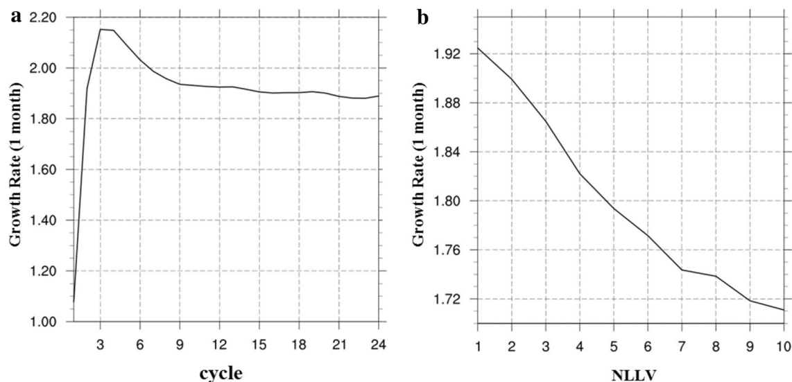
Fig. 4 The growth rate of the SSTA field of the NLLV1 as a function of the number of breeding cycles ( a ) and the growth rate of the first ten NLLVs through 12 breeding cycles ( b ). Here, the error growth rate is the average from the 408.5th to 3408.5th months. a Shows
